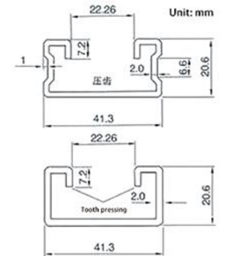
SOLAR PV BRACKETS
